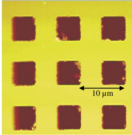
Figure 20: 10 \mu\text{m} AFM calibration standard (AFM image)
